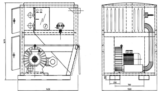
Layout CVU 11/16,5 kW
